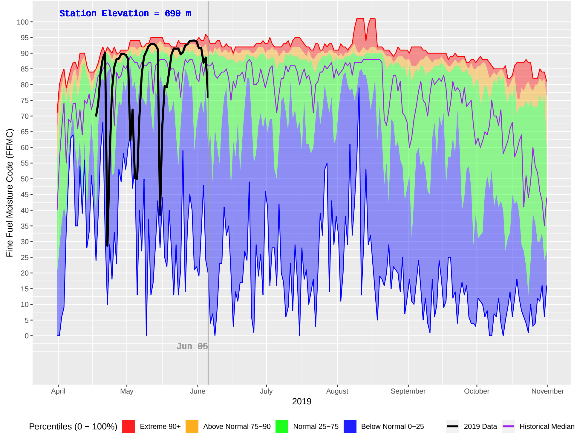
MACKENZIE FS (155) : Historical (1994–2018) and Current (2019) Daily Fine Fuel Moisture Code (FFMC)
