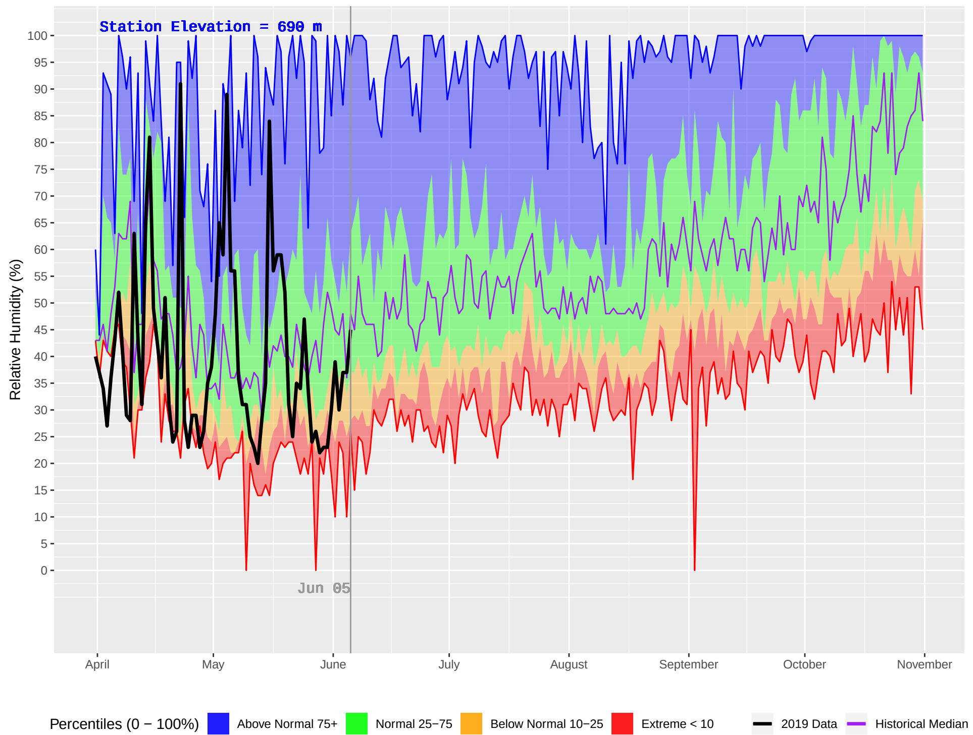
MACKENZIE FS (155) : Historical (1994–2018) and Current (2019) Daily Relative Humidity
