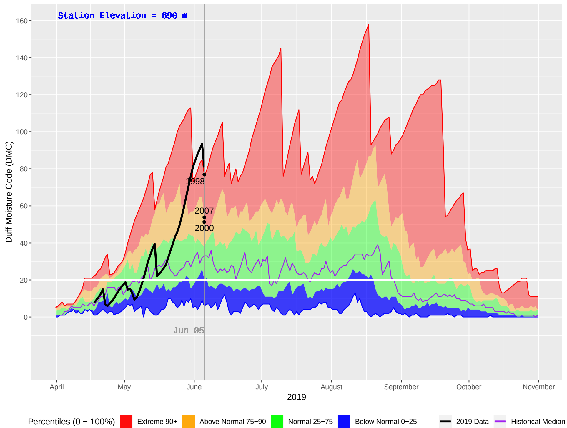
MACKENZIE FS (155) : Historical (1994–2018), Current (2019) Daily Duff Moisture Code (DMC)
