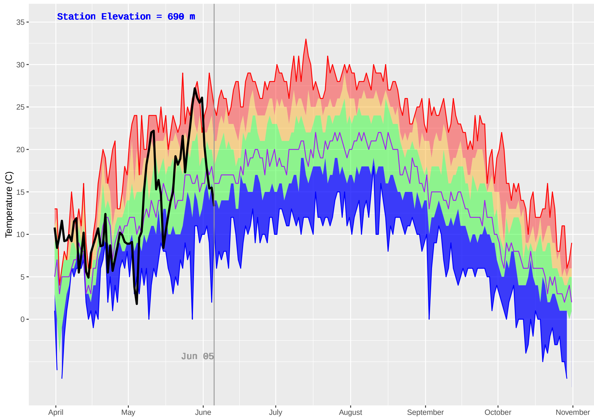
MACKENZIE FS (155) : Historical (1994–2018) and Current (2019) Daily Temperature
