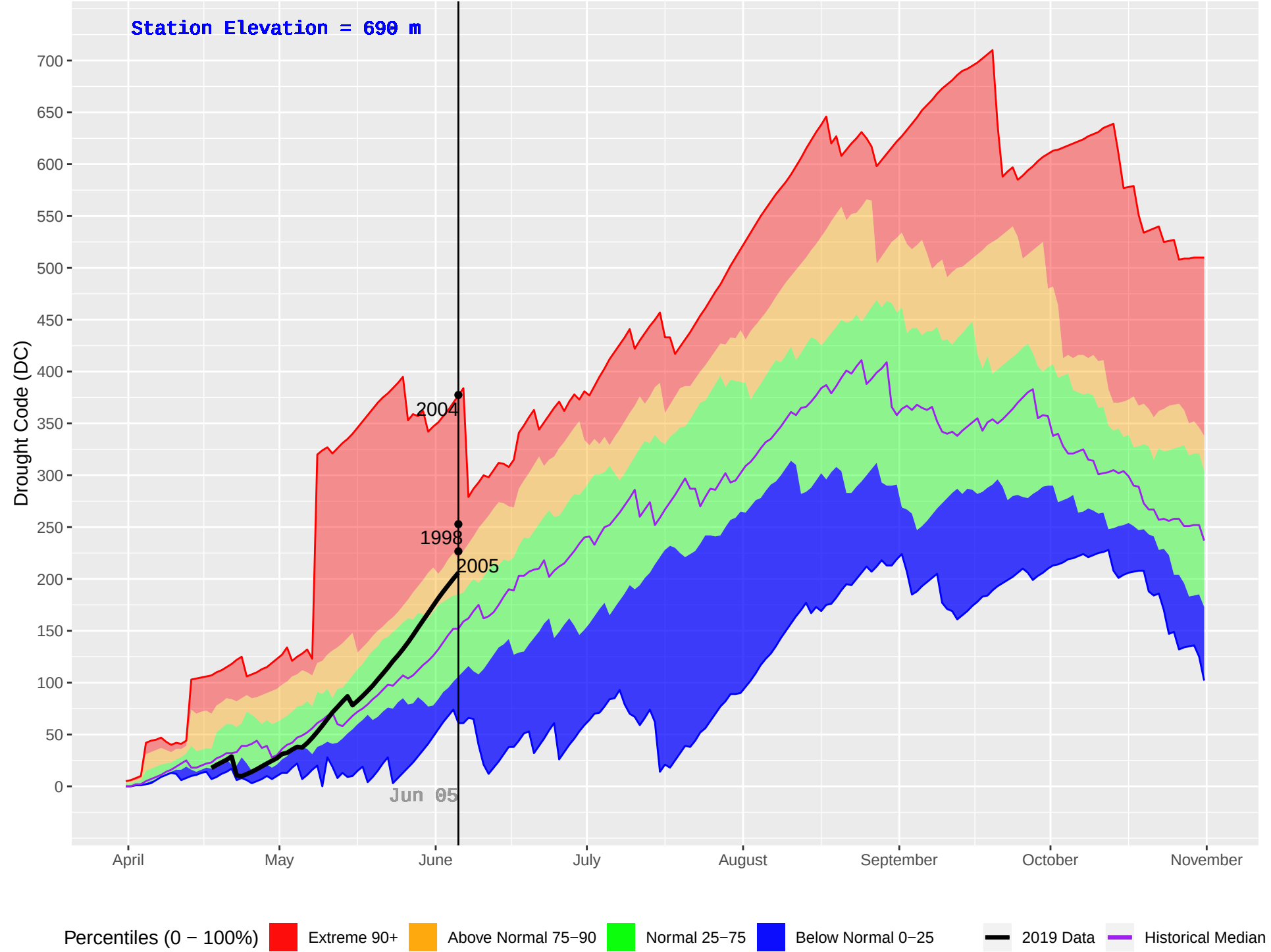
MACKENZIE FS (155) : Historical (1994–2018) and Current (2019) Daily Drought Code (DC)
