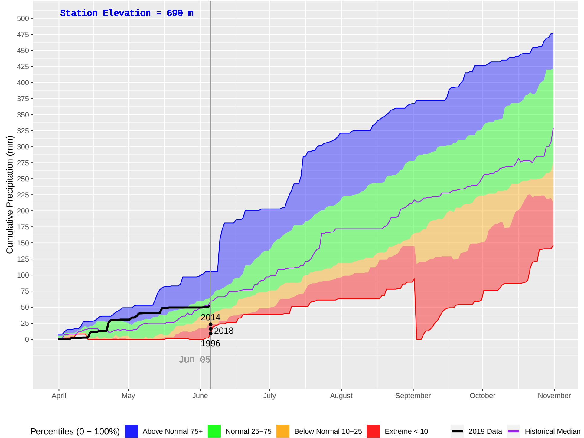
MACKENZIE FS (155) : Historical (1994–2018), Current (2019) Daily Cumulative Precipitation
