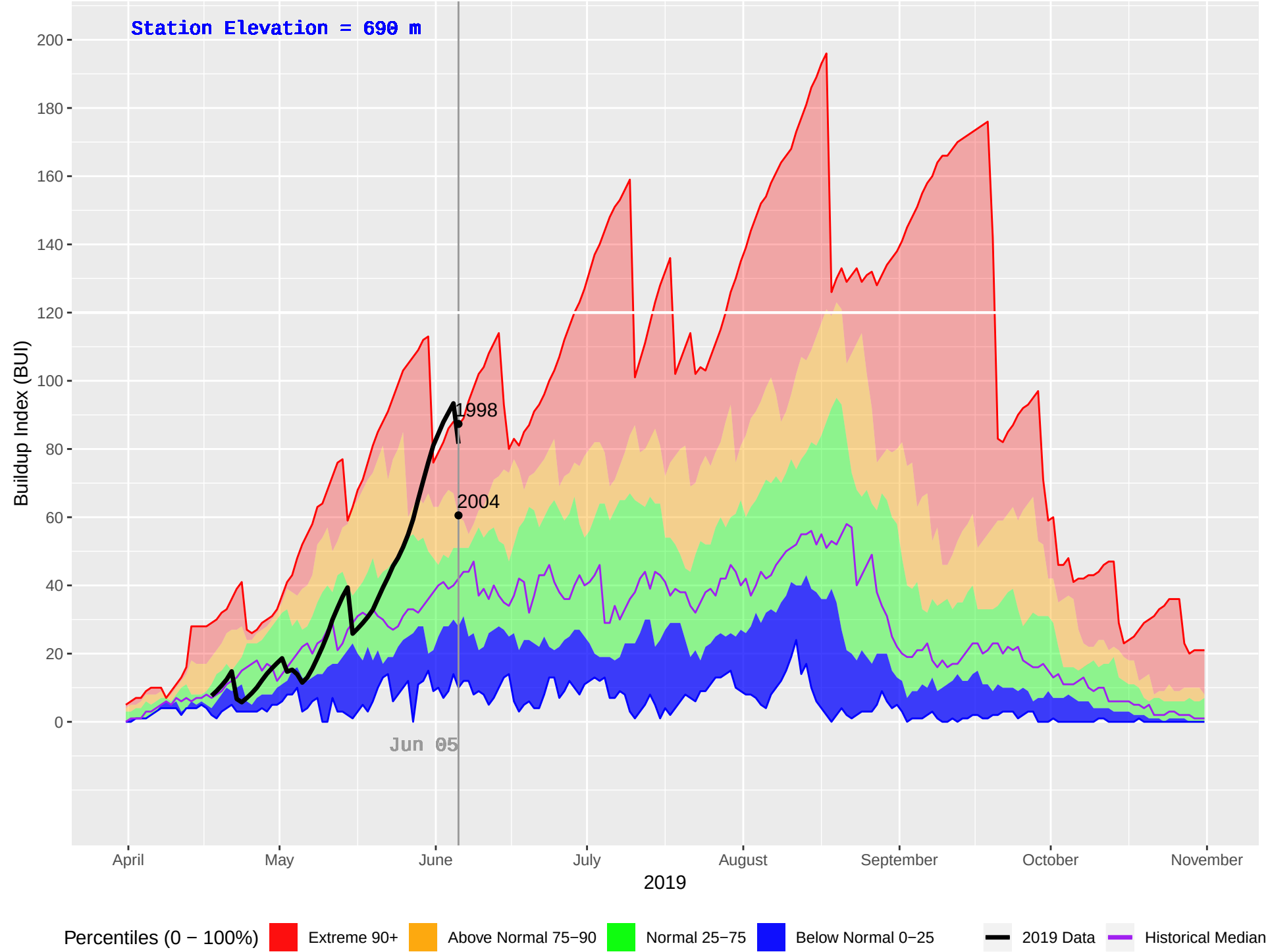
MACKENZIE FS (155) : Historical (1994–2018), Current (2019) Daily Buildup Index (BUI)
